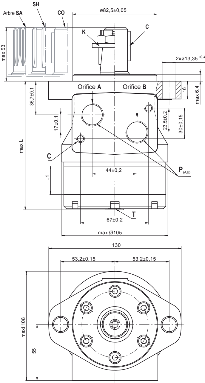
Fixation ovale (2 trous)
