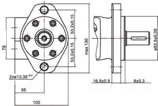
Fixation ovale (2 trous)
