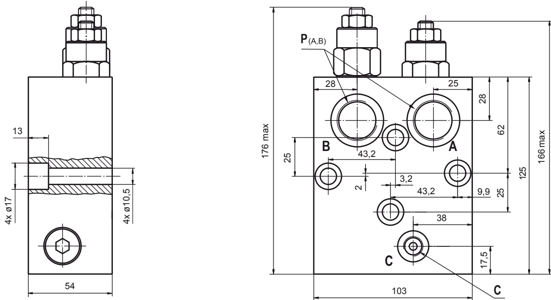
➤ Valve double KPBT-250/1/D...
