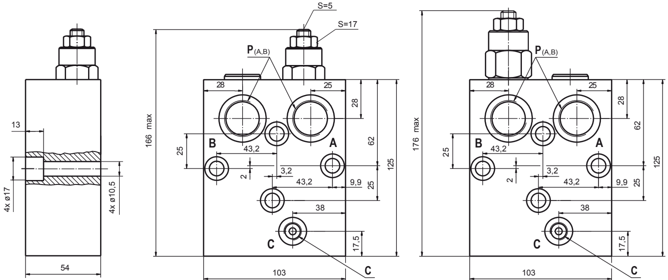
➤ Valve simple KPBT-250/1/E...
