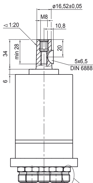
Arbre type "K1"
