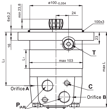
MSS - Montage court
