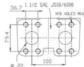
Raccordement GS
